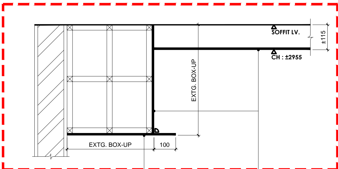
CEILING DETAIL SECTION S3 SCALE 1:10
