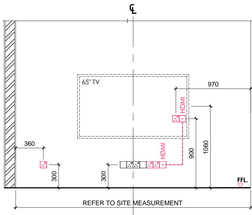
ELEVATION OF LIVING AREA SCALE 1 : 30
