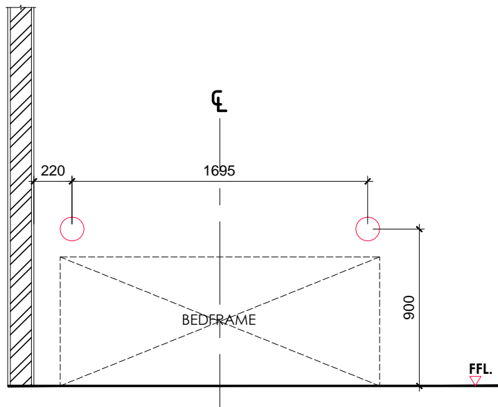
DETAIL OF WALL LIGHT @ MASTER BEDROOM SCALE 1 : 30
