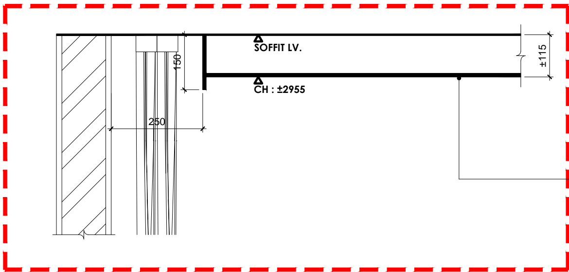
CEILING DETAIL SECTION S1 SCALE 1:10
