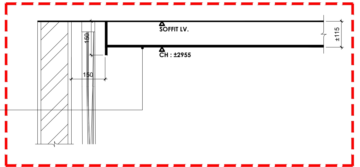
CEILING DETAIL SECTION S2 SCALE 1:10
