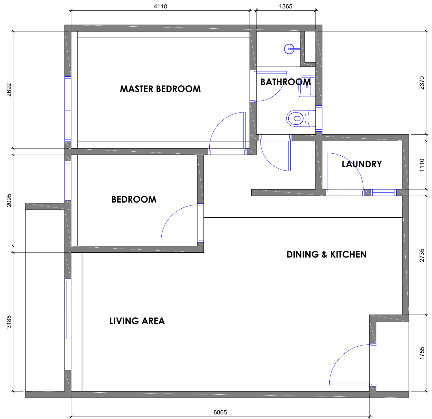
HABITUS APARTMENT LAYOUT PLAN SCALE 1 : 50 (A3) 586 sqft.
