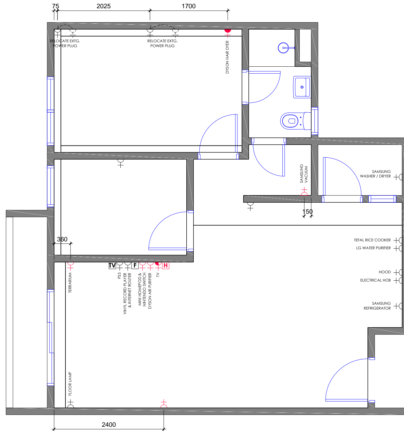
HABITUS APARTMENT ELECTRICAL LAYOUT PLAN SCALE 1 : 50 (A3) 586 sqft.
