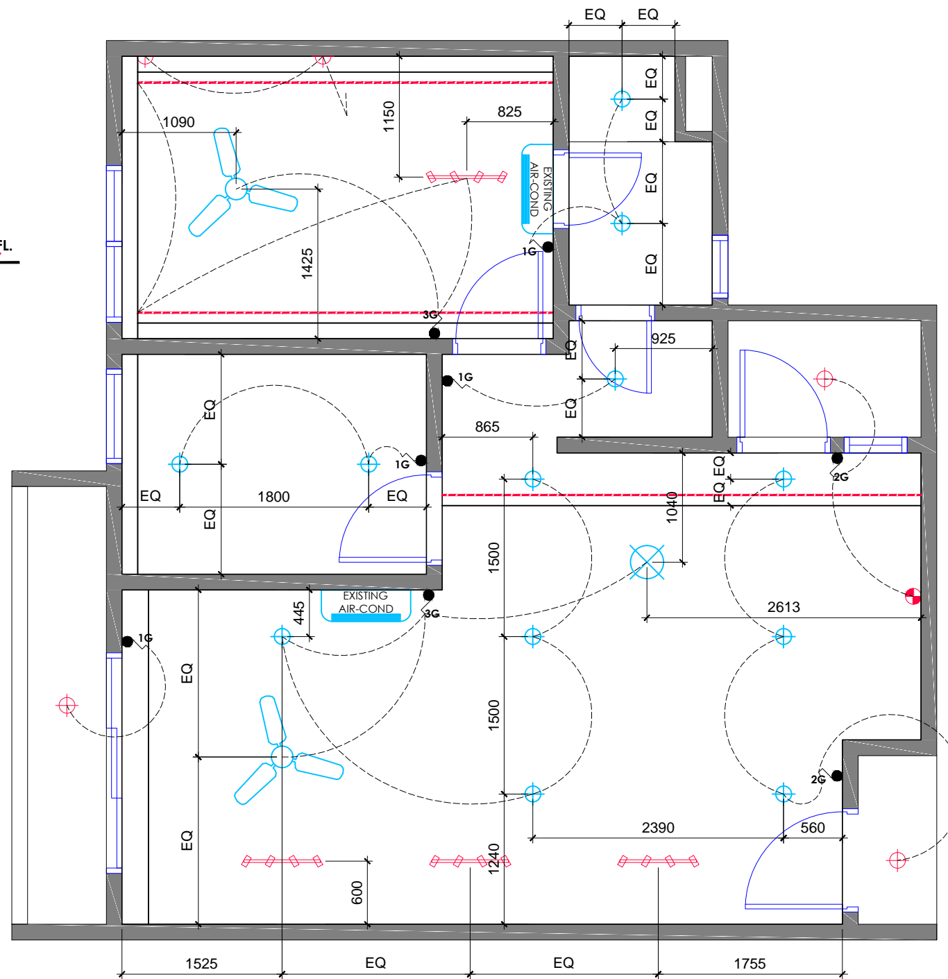
HABITUS APARTMENT REFLECTED CEILING PLAN SCALE 1 : 50 (A3) 586 sqft.
