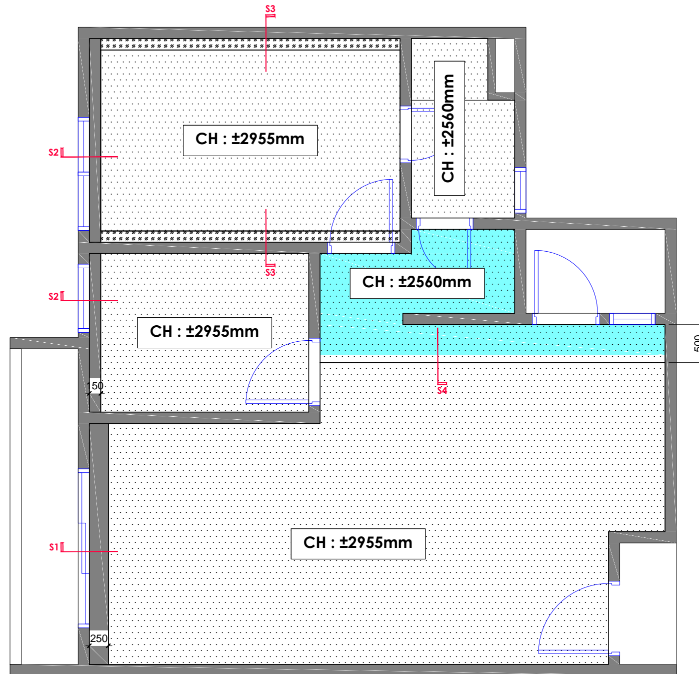
HABITUS APARTMENT CEILING FINISHES LAYOUT PLAN SCALE 1 : 50 (A3) 586 sqft.
