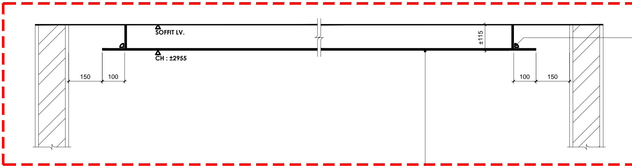
CEILING DETAIL SECTION S3 SCALE 1:10
