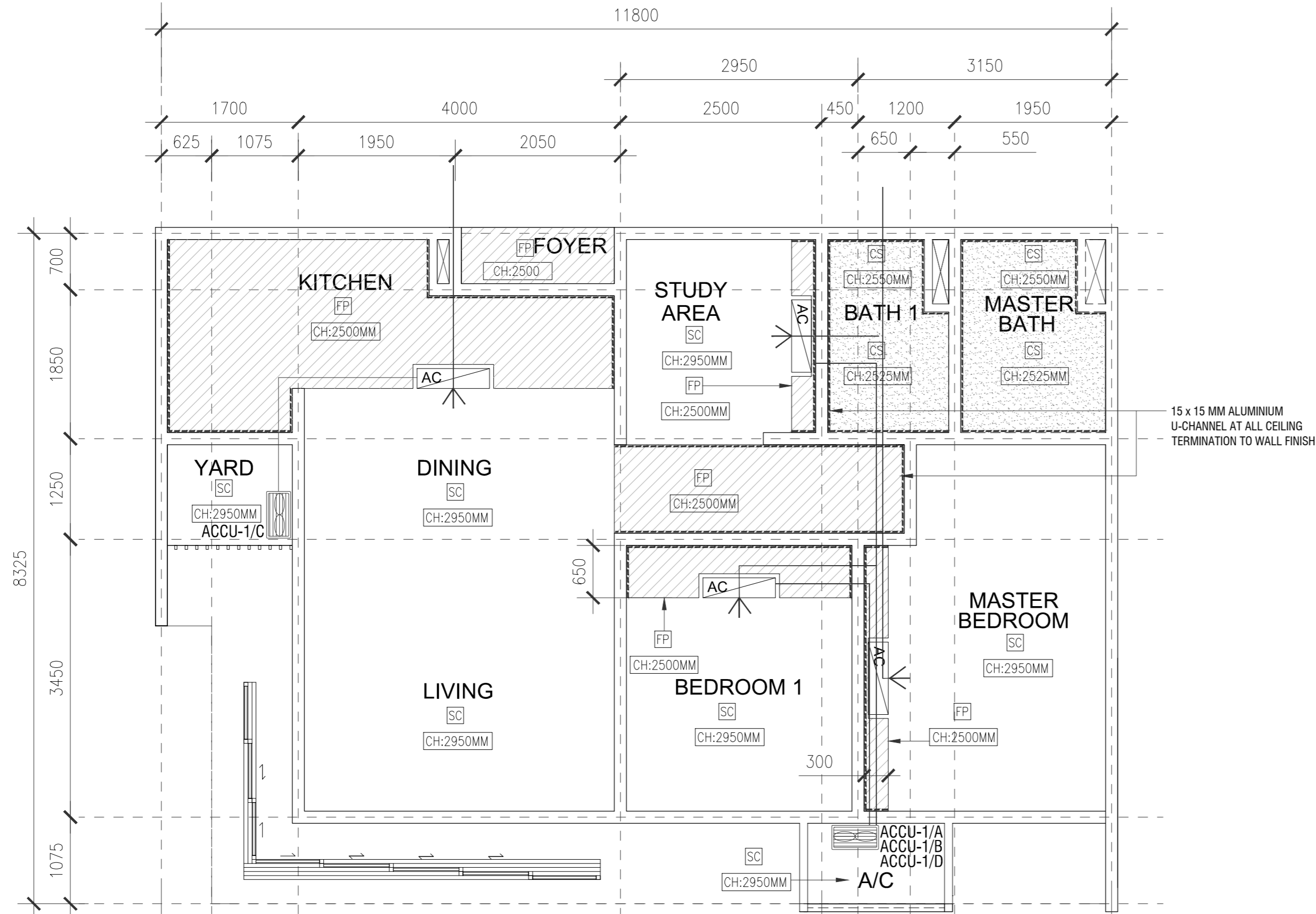
REFLECTED CEILING LAYOUT DETAIL. SCALE 1 : 50 TYPICAL TYPE B ( 850 ) - REFLECTED FLOOR PLAN - AIRCOND AND SPRINKLER LAYOUT
