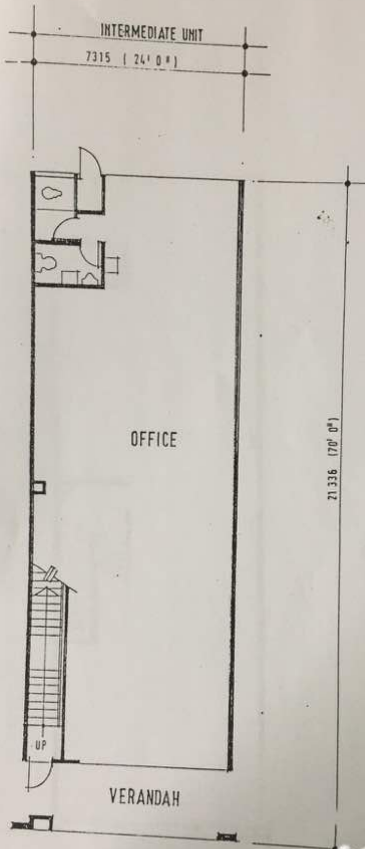
GROUND FLOOR PLAN (TYPE C)
